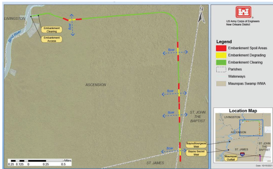
Figure 4. Embankment
